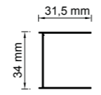
Profilo a parete_Wall profile Profilé mural_Wandprofil
