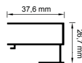
Profilo a parete_Wall profile Profilé mural_Wandprofil
